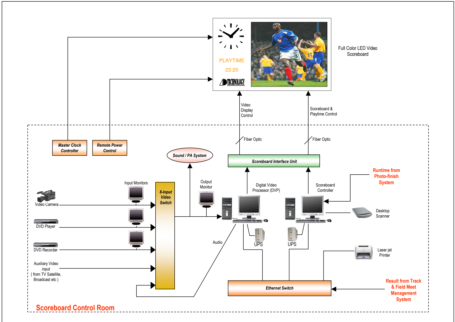
FULL COLOUR LED VIDEO SCOREBOARD SYSTEM SCHEMATICS
