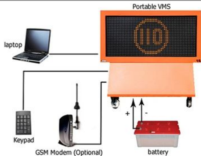
Portable Variable Message Sign System Schematics
