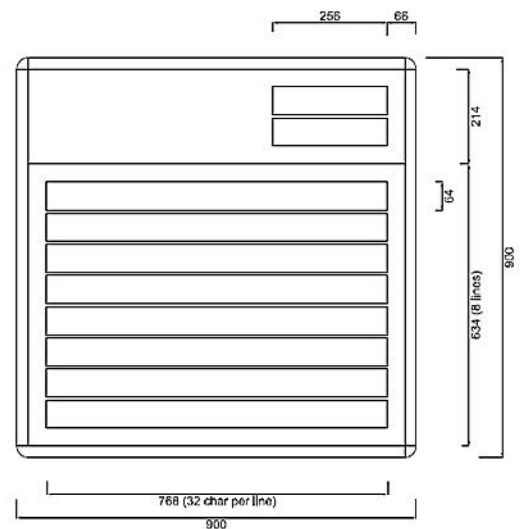
Type 1: Multi Lines
