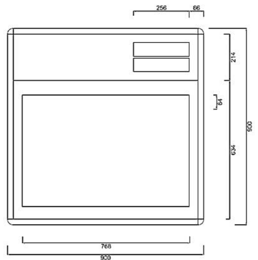
Type 2: Full Matrix
